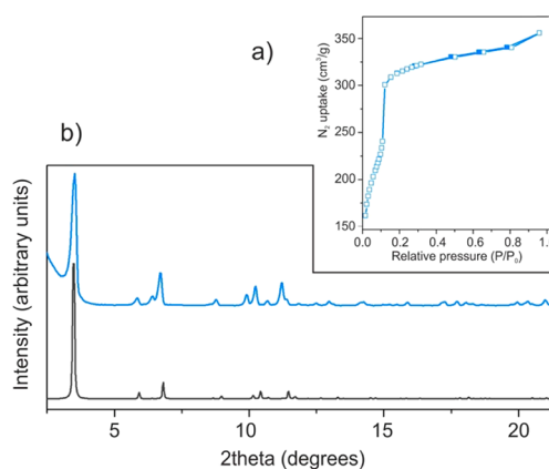
Figure 3. (a) N_2 adsorption isotherm of InPF-110. Empty and filled symbols represent adsorption and desorption points, respectively. (b) Calculated and experimental PXRD patterns for InPF-110 calcd (gray), InPF-110 expt (blue).
