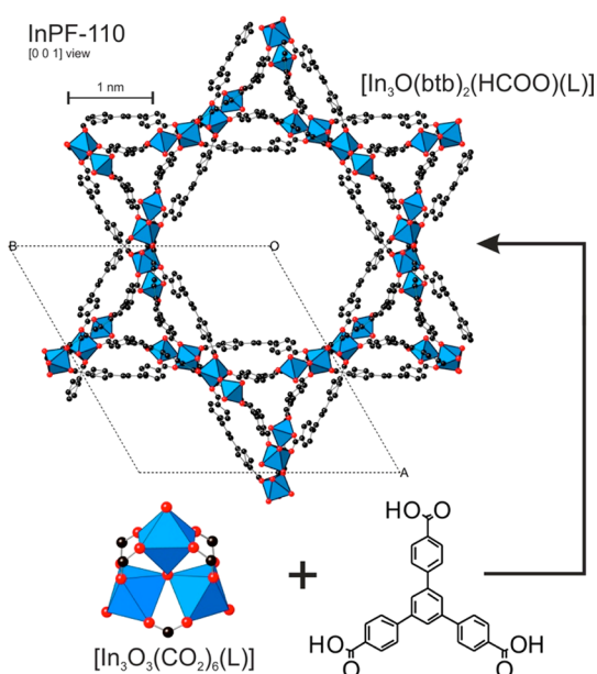
Figure 1. H_3btbt linker is combined with a trimeric In-SBU to produce InPF-110. C is black, O is red, and In atoms are blue polyhedra. L = solvent ligand (water, methanol, ethanol).
